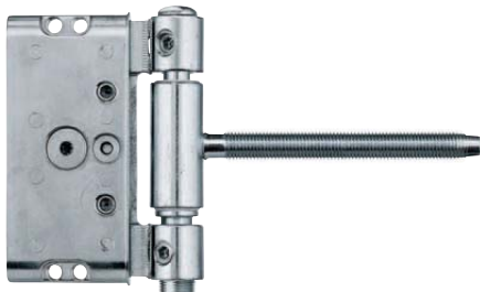
Duplex 320-3D-TGB S1
